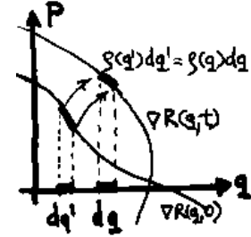
Figure 33.2: Density evolution of an initial surface (q', p' = \partial_q R(q', 0)) into (q(t), p(t)) surface time t later, sketched in 1 dimension. While the number of trajectories and the phase space Liouville volume are conserved, the density of trajectories projected on the q coordinate varies; trajectories which started in dq' at time zero end up in the interval dq .
