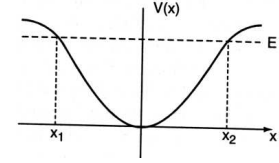
Figure 32.1: A 1-dimensional potential, location of the two turning points at fixed energy E .
