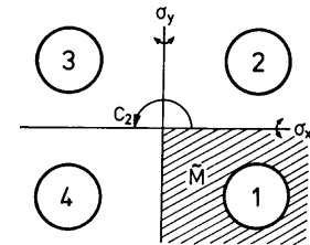
Figure H.2: Symmetries of four disks on a rectangle. A fundamental domain indicated by the shaded wedge.
