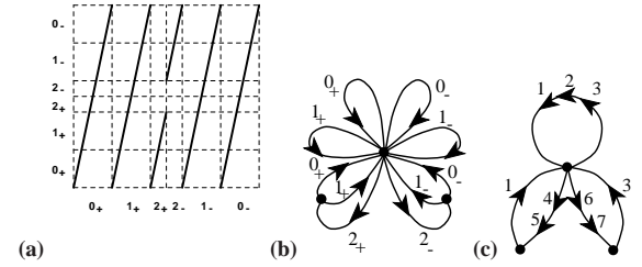
Figure 25.4: (a) A partition of the unit interval into six intervals, labeled by the jumping number \hat{h}(x) I = \{0_+, 1_+, 2_+, 2_-, 1_-, 0_-\} . The partition is Markov, as the critical point is mapped onto the right border of \mathcal{M}_{1_+} . (b) The transition graph for this partition. (c) The transition graph in the compact notation of (25.26) (introduced by Vadim Moroz).
