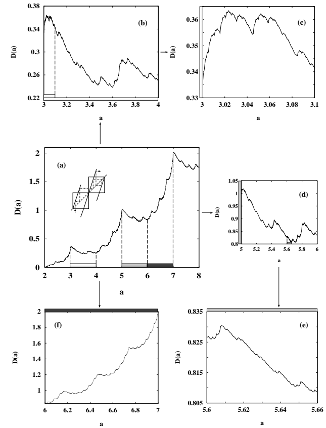
Figure 25.5: The dependence of D on the map parameter a is continuous, but not monotone. Here a stands for the slope \Lambda in (25.9). (From ref. [25.9].)
