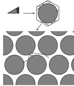
Figure 25.2: Tiling of \hat{\mathcal{M}} , a periodic lattice of reflecting disks, by the fundamental domain \tilde{\mathcal{M}} . Indicated is an example of a global trajectory \tilde{x}(t) together with the corresponding elementary cell trajectory x(t) and the fundamental domain trajectory \tilde{x}(t) . (Courtesy of J.-P. Eckmann)
