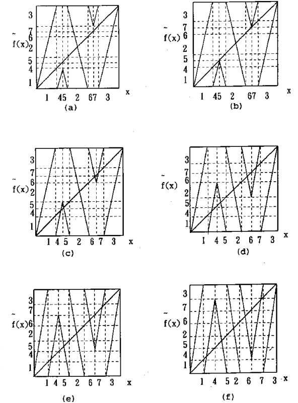
Figure S.1: (a)-(f) The sawtooth map (S.1) for the 6 values of parameter a for which the folding point of the map aligns with the endpoint of one of the 7 intervals and yields a finite Markov partition (from ref. [S.1]). The corresponding transition graphs are given in figure S.2.
