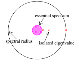
Figure 21.4: Spectrum of the Perron-Frobenius operator acting on the space of \mathbb{C}^{k+\alpha} Hölder-continuous functions: only k isolated eigenvalues remain between the spectral radius, and the essential spectral radius which bounds the “essential,” continuous spectrum.
