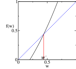
Figure 21.1: A nonlinear one-branch repeller with a single fixed point w^* .
