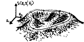
Figure 33.2: A romanticized sketch of S_p(E) = S(q, q, E) = \oint p(q, E) dq landscape orbit. Unstable periodic orbits traverse isolated ridges and saddles of the mountainous landscape of the action S(q_{||}, q_{\perp}, E) . Along a periodic orbit S_p(E) is constant; in the transverse directions it generically changes quadratically.
