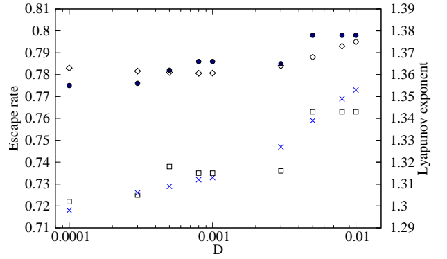
FIG. 3: (left scale) the escape rate of the repeller (9) vs. the noise strength D , calculated using (□) the ‘optimal partition’, and (×) a uniform discretization (16) in N = 128 intervals; (right scale) the Lyapunov exponent of the same repeller vs. D , estimated using (●) the ‘optimal partition’, and (◇) the average (17).
