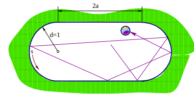
Fig. 8.1 The stadium billiard is a 2-dimensional domain bounded by two semi-circles of radius d = 1 connected by two straight walls of length 2a . At the points where the straight walls meet the semi-circles, the curvature of the border changes discontinuously; these are the only singular points of the flow. The length a is the only parameter.
