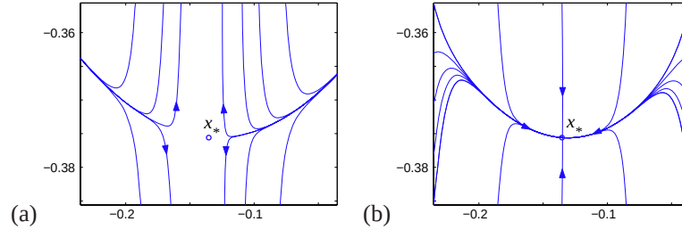
Fig. 27.4 Typical trajectories of the vector field (27.10) for a hyperbolic fixed point (x, y) \approx (-0.13529, -0.37559) of f^3 , where f is the Ikeda map (27.11). The circle indicates the position of the fixed point. For the vector field corresponding to (a) \mathbf{C} = \mathbf{1} , x_* is a hyperbolic equilibrium point of the flow, while for (b) \mathbf{C} = \begin{pmatrix} 1 & 0 \\ 0 & -1 \end{pmatrix} , x_* is an attracting equilibrium point.
