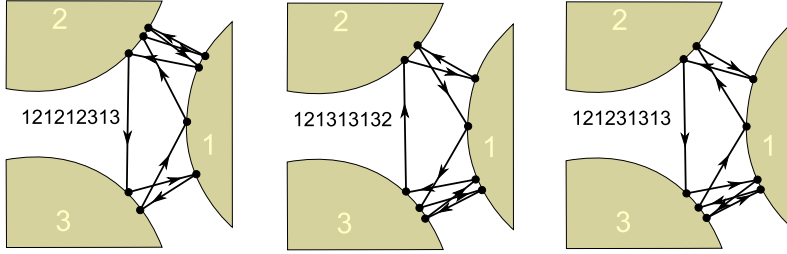
Fig. 9.7 Cycle \overline{121212313} has multiplicity 6; shown here is \overline{121313132} = \sigma_{23}\overline{121212313} . However, \overline{121231313} which has the same stability and period is related to \overline{121313132} by time reversal, but not by any C_{3v} symmetry.
