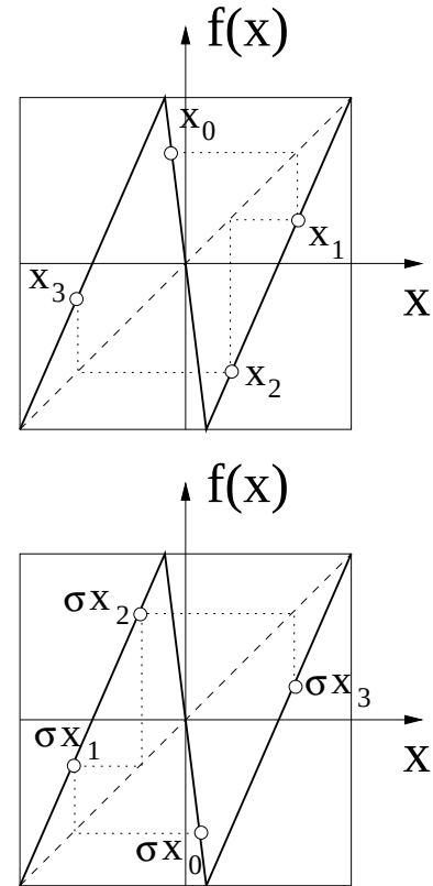
Fig. 9.1 The bimodal Ulam sawtooth map with the D_1 symmetry f(-x) = -f(x) . If the trajectory x_0 \rightarrow x_1 \rightarrow x_2 \rightarrow \dots is a solution, so is its reflection \sigma x_0 \rightarrow \sigma x_1 \rightarrow \sigma x_2 \rightarrow \dots . (continued in Fig. 9.2)
