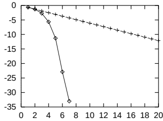
Fig. 13.4 Convergence of Newton method ( \diamond ) vs. inverse iteration ( + ). The error after n iterations searching for the \overline{01} -cycle of the logistic map f(x) = 4x(1-x) with an initial starting guess of x_1 = 0.2, x_2 = 0.8 . y-axis is \log_{10} of the error. The difference between the exponential convergence of the inverse iteration method and the super-exponential convergence of Newton method is dramatic.
