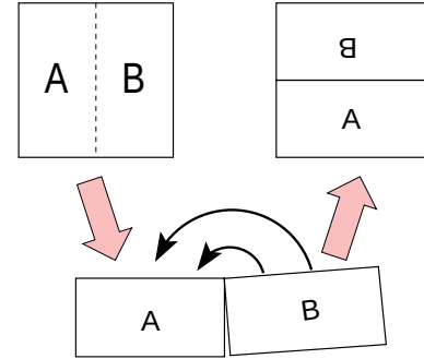
Fig. 12.5 Kneading orientation preserving danish pastry: mimic the horseshoe dynamics of Fig. 12.6 by: (1) squash the unit square by factor 1/2, (2) stretch it by factor 2, and (3) fold the right half back over the left half.
