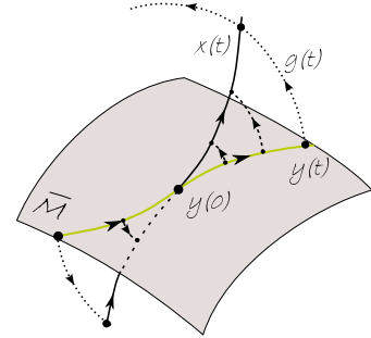
Fig. 10.10 Slice \bar{\mathcal{M}} is a Poincaré section (10.41) for group orbits (indicated by dotted lines here). The full state space trajectory x(t) and the reduced state space trajectory y(t) belong to the same group orbit \mathcal{M}_{k(t)} and are equivalent up to a group rotation g(t) (10.40).
