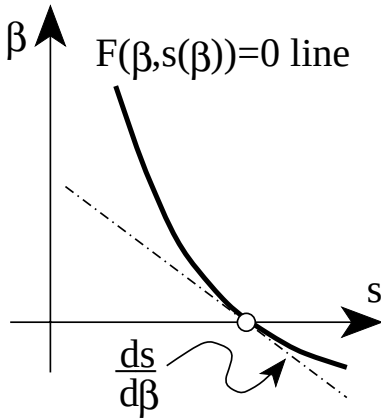
Fig. 20.2 The eigenvalue condition is satisfied on the curve F = 0 the (\beta, s) plane. The expectation value of the observable (17.12) is given by the slope of the curve.
