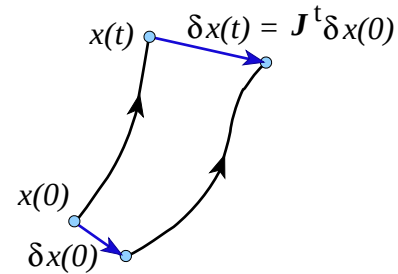
Fig. 1.10 The Jacobian matrix J^t maps an infinitesimal displacement \delta x at x_0 into a displacement J^t(x_0)\delta x finite time t later.
