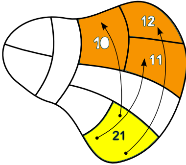
Fig. 14.1 Points from the region \mathcal{M}_{21} reach regions \{\mathcal{M}_{10}, \mathcal{M}_{11}, \mathcal{M}_{12}\} , and no other regions, in one time step. Labeling exemplifies the ‘shift map’ of Example 11.7 and (11.20).
