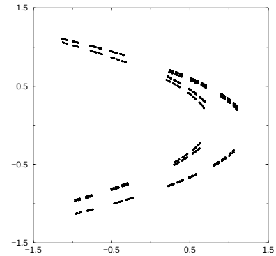
Fig. 27.2 The repeller for the Hénon map at a = 1.8 , b = 0.3 .
