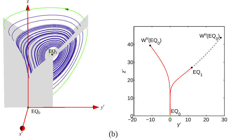
Fig. 11.8 (a) A Poincaré section of the Lorenz flow in the doubled-polar angle representation, Fig. 9.4, given by the [y', z] plane that contains the z -axis and the equilibrium EQ_1 . The x' axis points toward the viewer. (b) The Poincaré section of the Lorenz flow by the section. Crossings into the section are marked red (solid) and crossings out of the section are marked blue (dashed). Outermost point of both in- and out-sections are given by the EQ_0 unstable manifold W^u(EQ_0) intersections. (E. Siminos)
