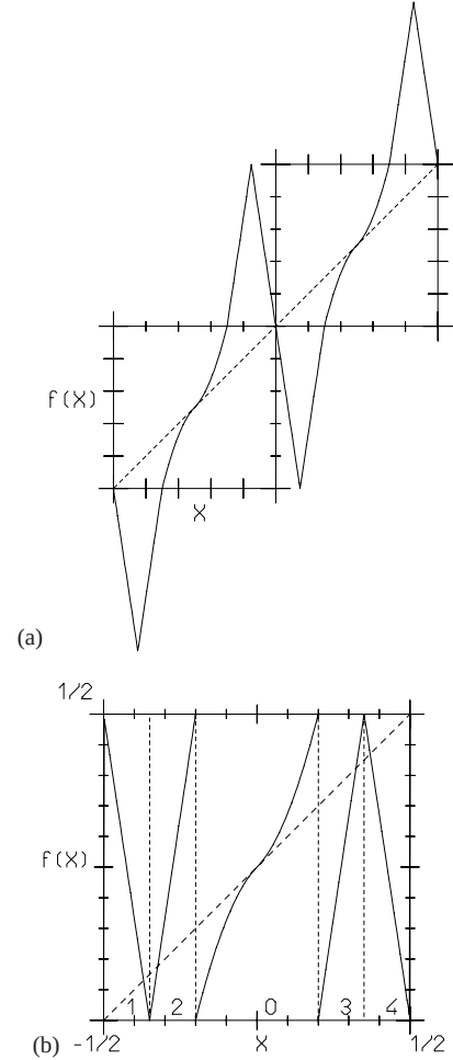
Fig. 25.6 (a) A map with marginal fixed point. (b) The map restricted to the unit circle. remark 25.7
