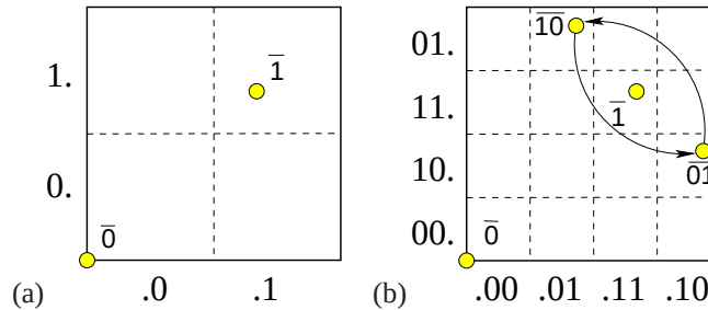
Fig. 12.7 Kneading danish pastry: symbol square representation of an orientation preserving once-folding map obtained by fattening the Smale horseshoe intersections of (a) Fig. 12.6 (b) Fig. 12.4 into a unit square. Also indicated: the fixed points \bar{0}, \bar{1} and the 2-cycle points \{\bar{01}, \bar{10}\} . In the symbol square the dynamics maps rectangles into rectangles by a decimal point shift.
