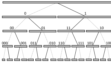
Fig. 11.14 Alternating binary tree relates the itinerary labeling of the unimodal map intervals, Fig. 11.12, to their spatial ordering. Dotted line stands for 0, full line for 1; the binary sub-tree whose root is a full line (symbol 1) reverses the orientation, due to the orientation reversing fold in Figs. 11.10 and 11.12. See also Fig. 14.4.
