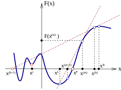
Fig. 13.5 Newton method: bad initial guess x^{(b)} leads to the Newton estimate x^{(b+1)} far away from the desired zero of F(x) . Sequence \dots, x^{(m)}, x^{(m+1)}, \dots , starting with a good guess converges super-exponentially to x^* . The method diverges if it iterates into the basin of attraction of a local minimum x^c .
