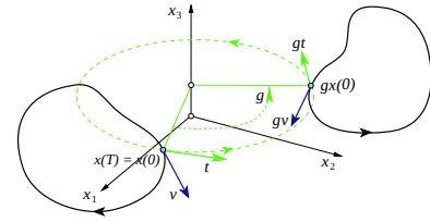
Fig. 10.5 A periodic orbit starts out at x(0) with the dynamical v and group tangent t flows pointing in different directions, and returns after time T_p to the initial point x(0) = x(T_p) . The group orbit of the temporal orbit of x(0) sweeps out a (1+N) -dimensional torus, a continuous family of equivalent periodic orbits, two of which are sketched here. For SO(2) this is topologically a 2-torus.
