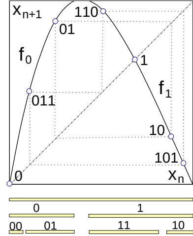
Fig. 11.12 A unimodal repeller with the survivor intervals after 1 and 2 iterations. Intervals marked s_1 s_2 \dots s_n consist of points that do not escape in n iterations, and follow the itinerary S^+ = s_1 s_2 \dots s_n . Note that the spatial ordering does not respect the binary ordering; for example x_{00} < x_{01} < x_{11} < x_{10} . Also indicated: the fixed points \bar{0} , \bar{1} , the 2-cycle \bar{01} , and the 3-cycle \bar{011} .
