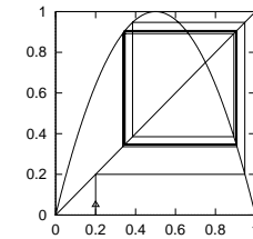
Figure 7.1: The inverse time path to the \overline{01} -cycle of the logistic map f(x) = 4x(1 - x) from an initial guess of x = 0.2 . At each inverse iteration we chose the 0 (respectively 1) branch.
