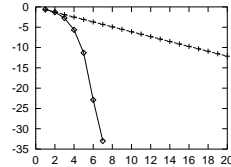
Figure 7.2: Convergence of Newton method ( \diamond ) vs. inverse iteration ( + ). The error after n iterations searching for the 01-cycle of the logistic map f(x) = 4x(1-x) with an initial starting guess of x_1 = 0.2, x_2 = 0.8 . The y-axis is \log_{10} of the error. The difference between the exponential convergence of the inverse iteration method and the super-exponential convergence of Newton method is dramatic.
