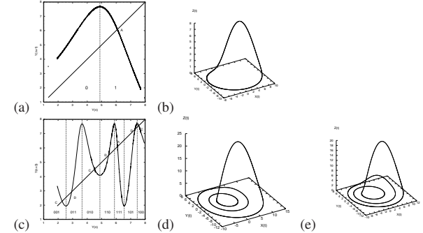
Figure 7.4: (a) The y \rightarrow P_1(y, z) return map for the x = 0, y > 0 Poincaré section of the Rössler flow figure 2.6. (b) The \bar{1} -cycle found by taking the fixed point y_{k+n} = y_k together with the fixed point of the z \rightarrow z return map (not shown) as an initial guess (0, y^{(0)}, z^{(0)}) for the Newton-Raphson search. (c) The third iterate, y_{k+3} = P_1^3(y_k, z_k) , of the Poincaré return map (3.1) together with the corresponding plot for z_{k+3} = P_2^3(y_k, z_k) , is used to pick initial guesses for the Newton-Raphson searches for the two 3-cycles: (d) the \overline{001} cycle, and (e) the \overline{011} cycle. (G. Simon)
